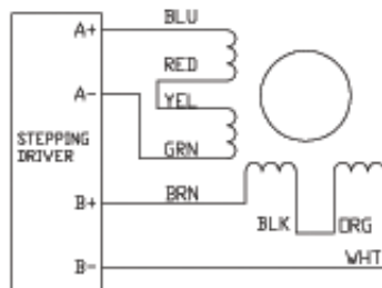
Bipolar Series
