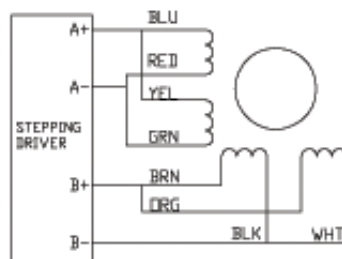
Bipolar Parallel
